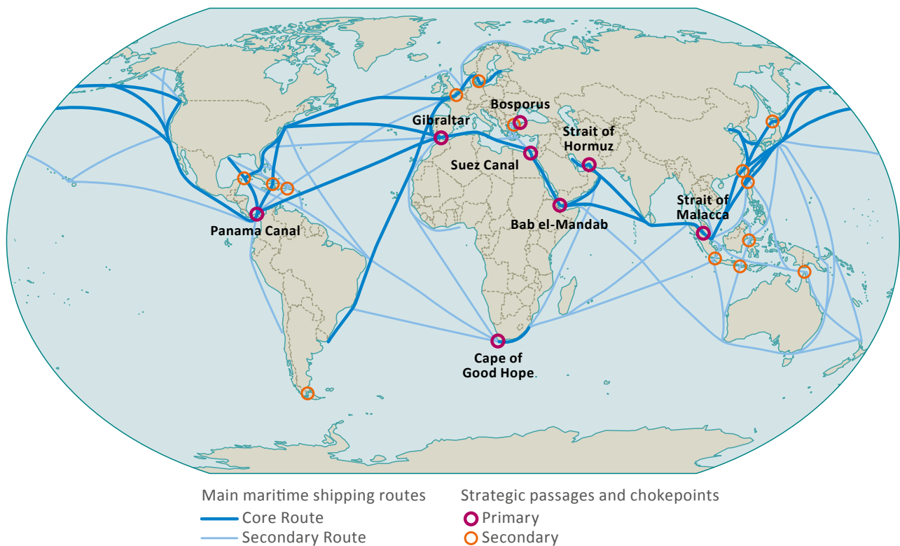
Figure 4: Global Maritime Shipping Routes
