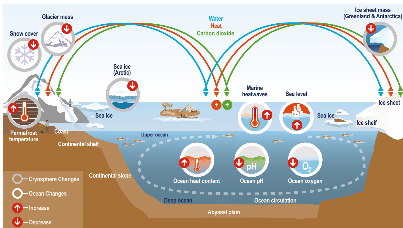
Figure 3: Key Components and Changes of the Ocean and Cryosphere
