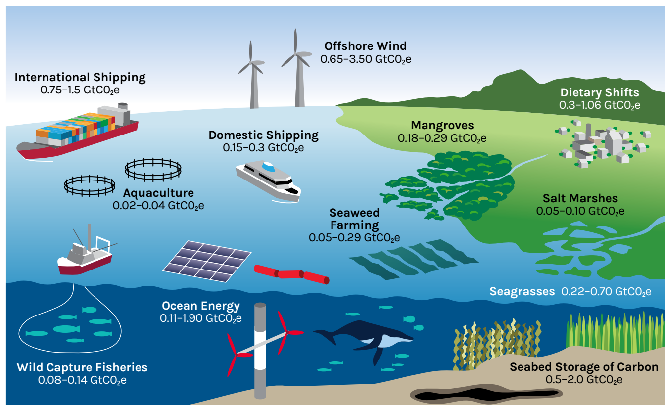
Figure 22: Ocean-based Mitigation Options
